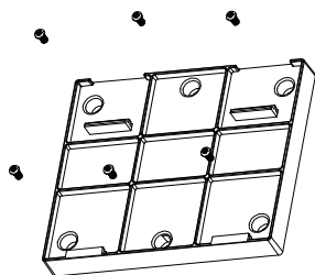
1 Mount the base panel on the wall with screws
