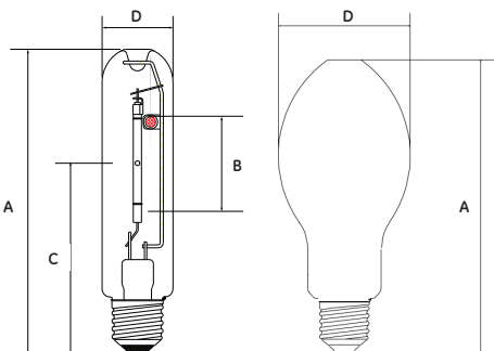
Lucalox™ XO - Elliptical Diffuse – Figure 2.
