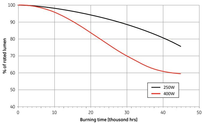
Lumen maintenance of XO 250-400W lamps
